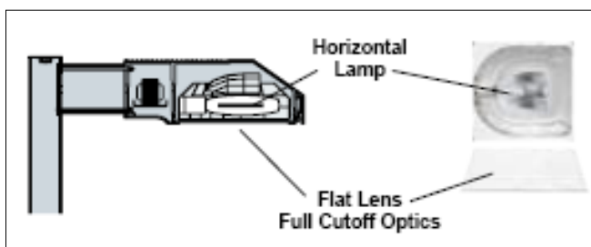
Photo B. Diagram of a full cut-off or concealed source fixture.
